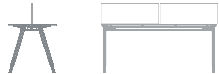
A-Extrusion Table (Side) L:1500 W:600 H:750
